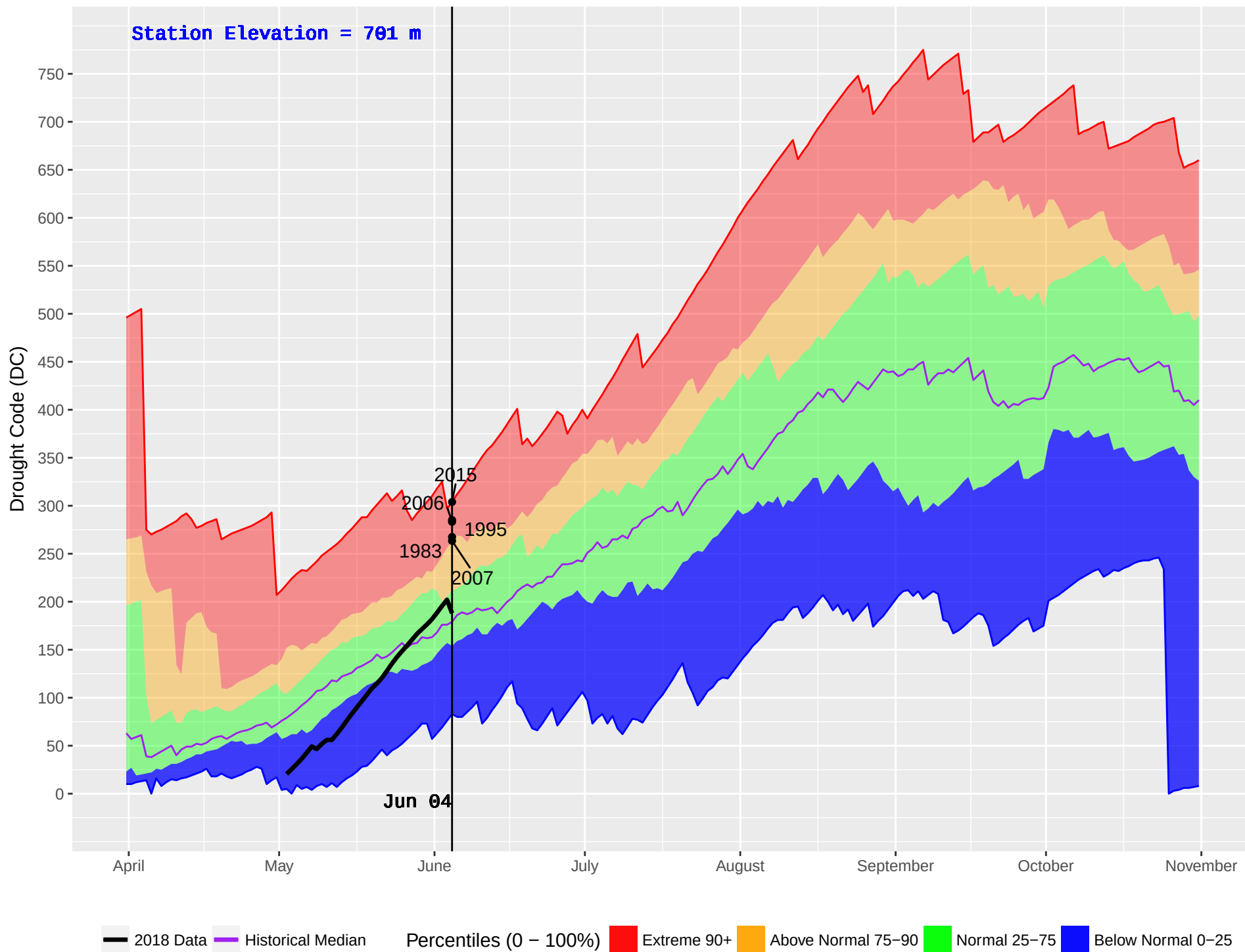
HORSEFLY (230) : Historical (1971–2016) and Current (2018) Noon Drought Code (DC)
