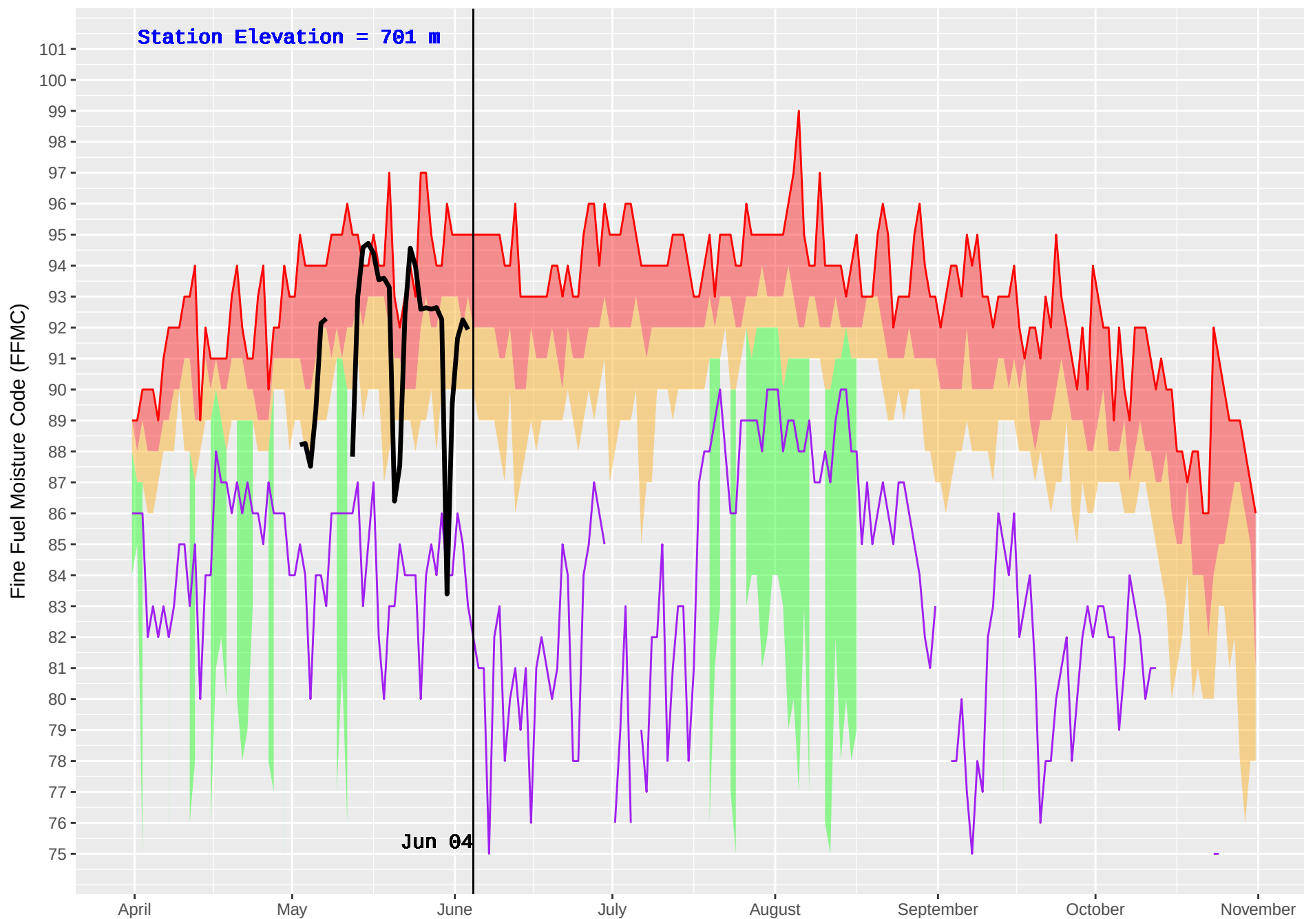
HORSEFLY (230) : Historical (1971–2016) and Current (2018) Noon Fine Fuel Moisture Code (FFMC)
